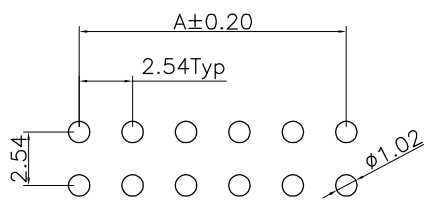
RECOMMENDED PCB LAYOUT (TOLERANCE:±0.05)
